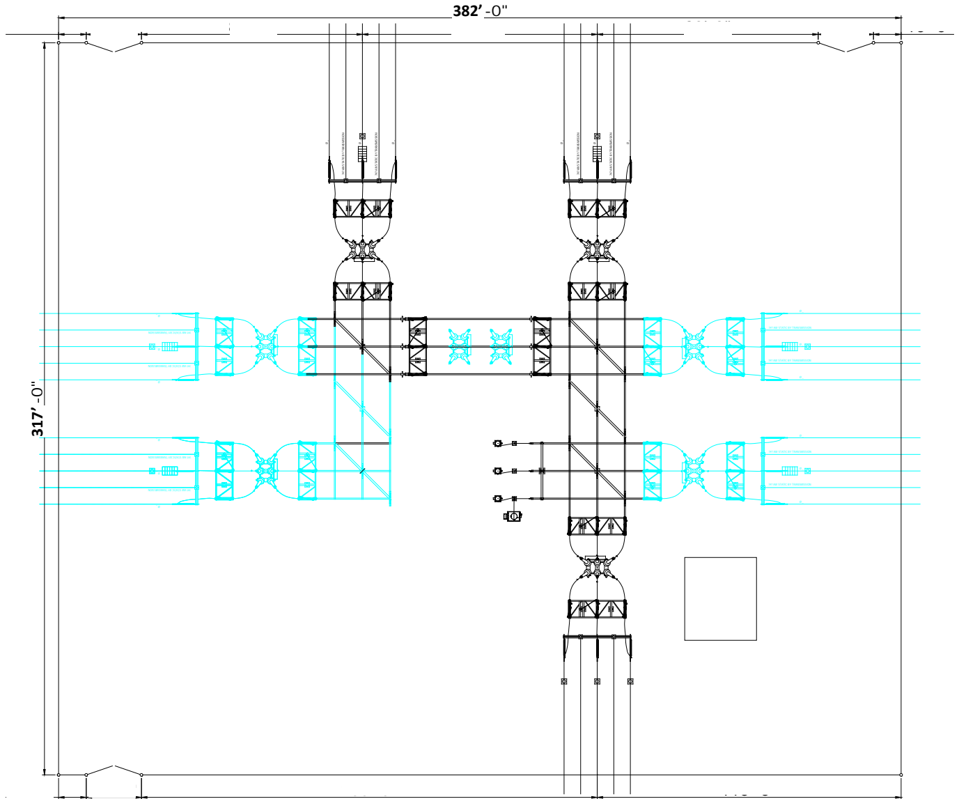
115 kV Three-Breaker Switching Station General Arrangement
